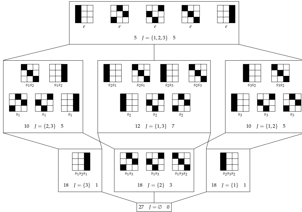
Figure 1: We take W = S_4 and \vec{c} = (s_1, s_2, s_3) and p = 3 . Each box is a set \mathcal{D}^J(\vec{c}^p) := \coprod_{v \in W^{l,+}} \mathcal{D}^{(v)}(\vec{c}^p) for some J . Edges between boxes are containments between J 's. Each \vec{\omega} \in \mathcal{D}^J(\vec{c}^p) is drawn as a 3 \times 3 box, with elements of \mathbf{e}_{\vec{\omega}} in black. For example, represents \vec{\omega} = (\text{id}, s_2, s_3, s_1, \text{id}, s_3, s_1, s_2, \text{id}) . In each box, the number to the left, resp. right, of J is the number of w \in W with \text{Des}(w) \supseteq J , resp. \text{Des}(w) = J . The former is \text{Park}_{W,p}^{J,+} . The rightmost number in the (k + 1) th row is \mathcal{P}_{2k}(L_{4,3})|_{\mathbf{v} \rightarrow 1} .
